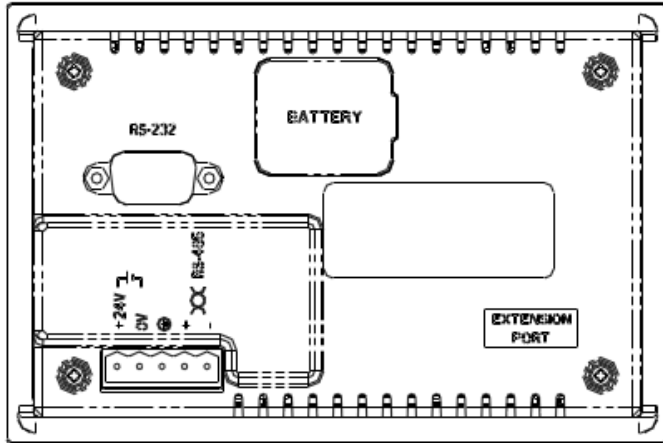
Arka panel
